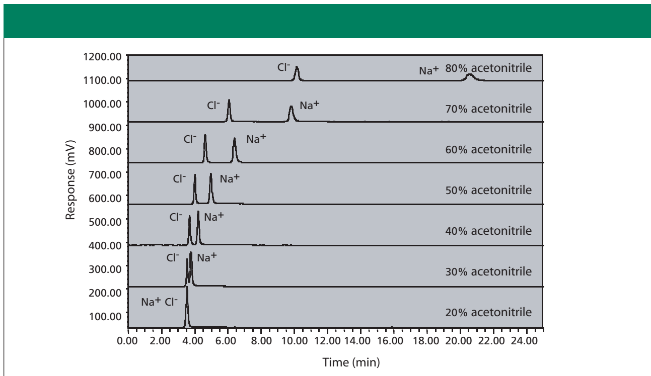
Figure 1: These chromatograms were generated at 75 mM ammonium acetate, pH 4.8 acetic acid. The organic content was varied from 20% to 80% acetonitrile. As % organic is increased, retention of both \text{Na}^+ and \text{Cl}^- were increased. This is consistent with HILIC.
