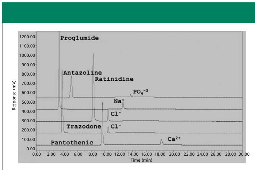
Figure 4: Overlay chromatograms of several pharmaceutical salts. In this example, the counterions are easily separated from each other. The molecules are separated from each other as well. Chromatography conditions are using 75 mM ammonium acetate buffer (pH 5.0) and the same gradient as described earlier. Salt forms are identified and quantitated in Table III.
