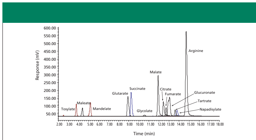
Figure 2: Overlay chromatogram of common organic ions used for pharmaceutical salt selection. Gradient was the same as Figure 1 with 75 mM ammonium acetate buffer (pH 3.8) concentration.
